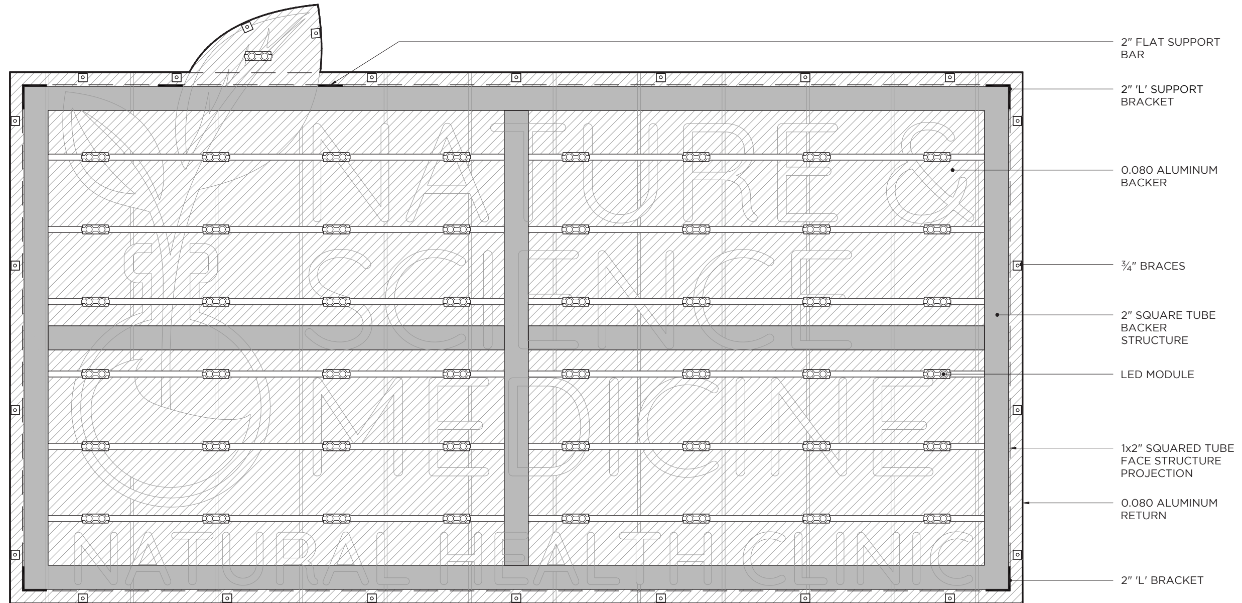
INTERNAL VIEW SCALE 1 1/2"=1'
